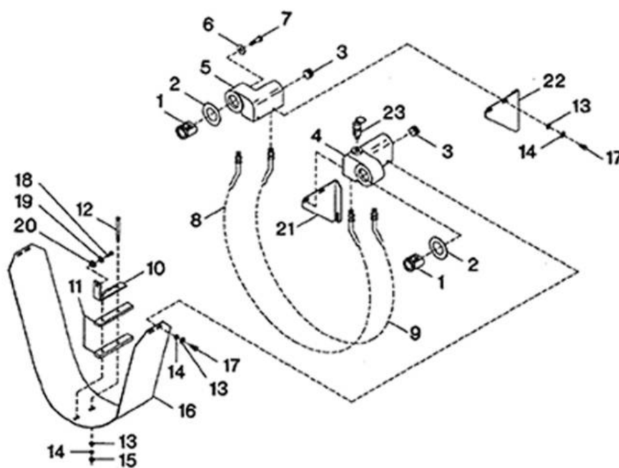
FIGURE 8. INTERCOOLER ASSEMBLY.
