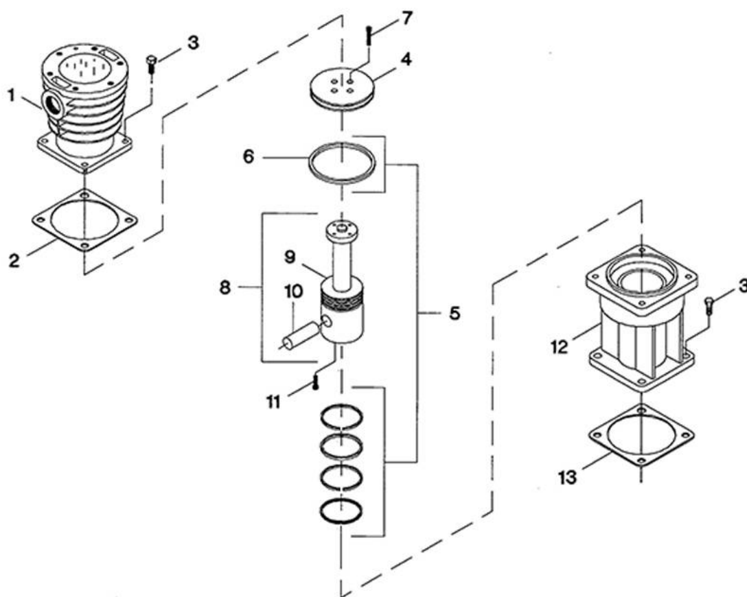
FIGURE 6. 5" PISTON, CYLINDER & CROSSHEAD
