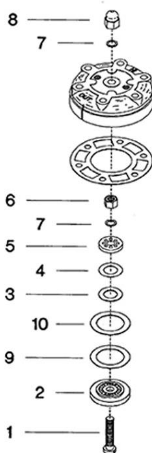
FIGURE 3. HIGH PRESSURE CONCENTRIC RING VALVE.
