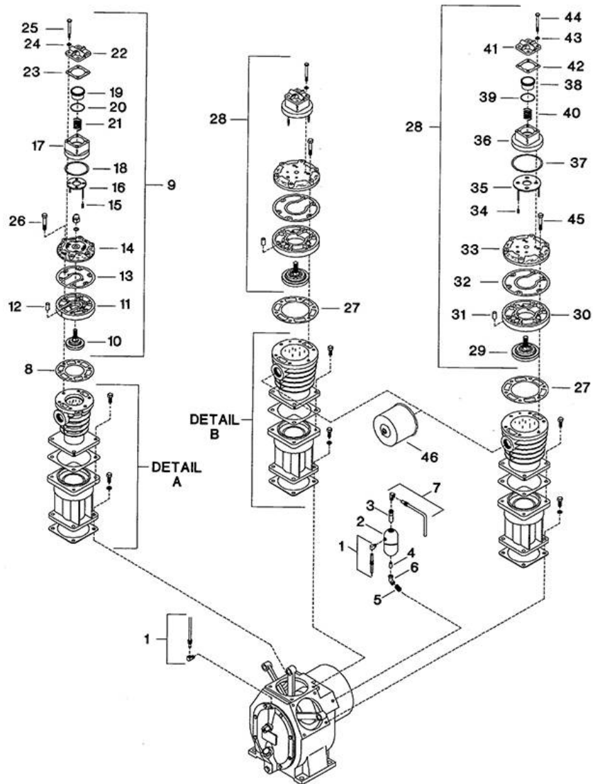
FIGURE 2. BARE COMPRESSOR.
